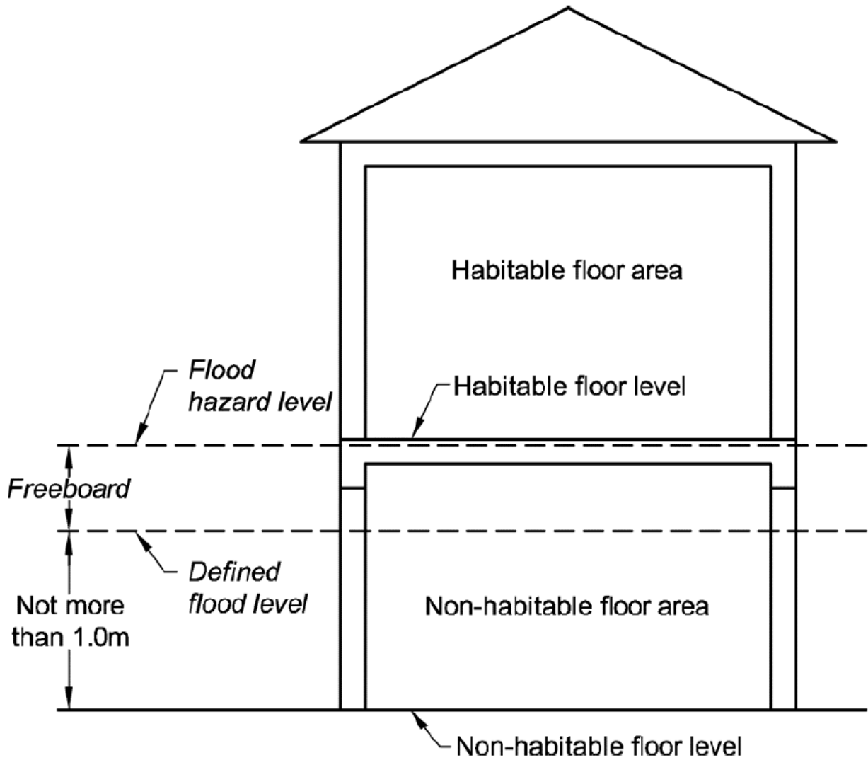
Figure 1 Identifying defined flood level (DFL) , flood hazard level (FHL) and freeboard
